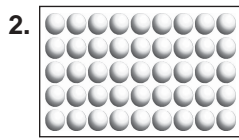
Molecules in a liquid
