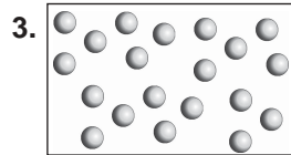
Molecules in a gas
