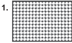
Molecules in a solid
